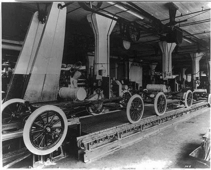
Unfinished Model T's rolling on the assembly line
